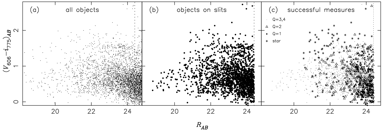
FIG. 10.— Apparent color-magnitude diagram for objects placed on TKRS masks. (a) The total sample of stars and galaxies in catalog; the dotted line represents the nominal limit of R_{AB} = 24.4 used in the selection of the spectroscopic sample. (b) The distribution of objects placed on masks. (c) Observed targets, including galaxies with secure redshifts ( Q = 3, 4 ), dubious measures ( Q = 2 ), objects for which no redshift can be measured ( Q = 1 ), and confirmed stars ( Q = -1 ). The Q = 1 sample generally consists of blue and faint objects, suggesting that these are likely to be high-redshift galaxies for which the [\text{O II}] \lambda\lambda 3726, 3729 lines fall outside the TKRS spectral window.
